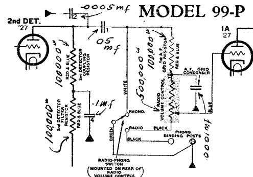
PHONOGRAPH SWITCHING CIRCUIT
